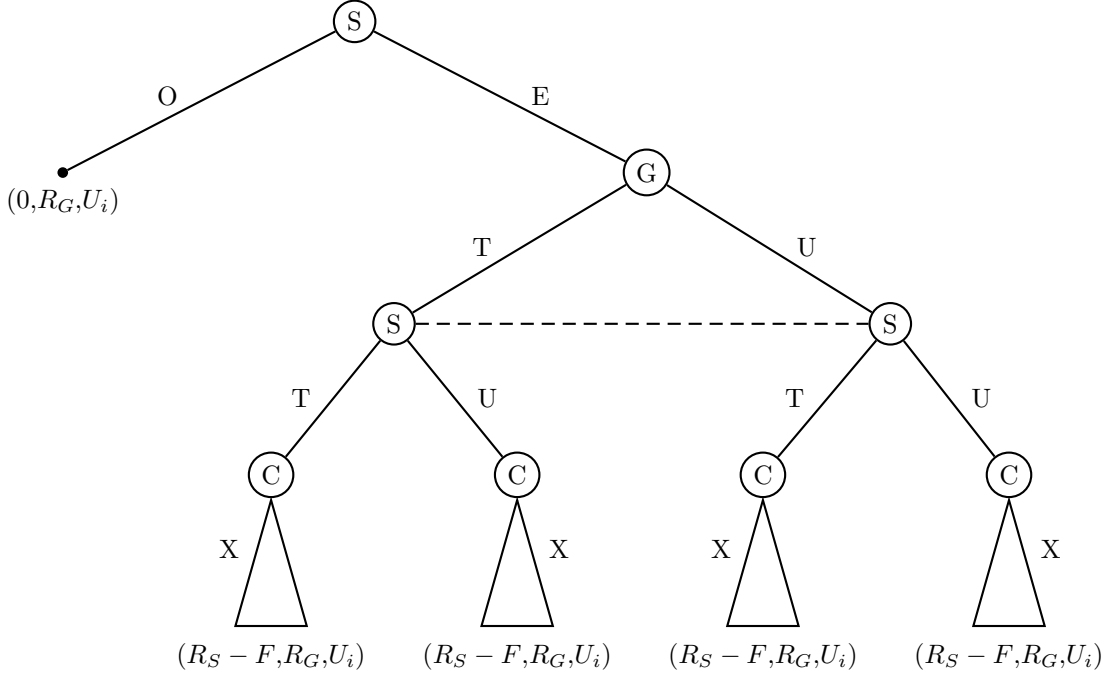
Figure 4: Extensive form
